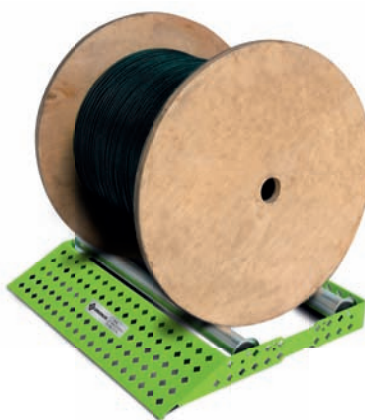
Easy Roller Broad (710 x 605 x 95 mm)
