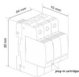
3 Poles
