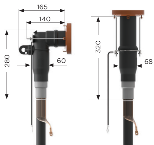
RSES VD: Elbow connector with test point
