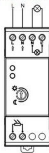
CIRCUIT DIAGRAM
