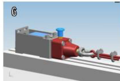
6- Make cable connections to the contact block. Before starting machine make sure that when the steel wire is pulled or broken , the contacts are activated . Reset the system
