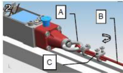
2-Fix steel wire (B) to switch ring (A) with clamps (C)
