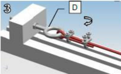
3- Fix the other side of the steel wire to pull stay bolt (D) with clamps.
